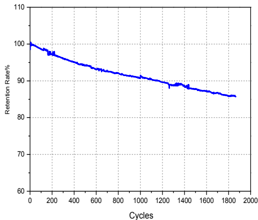
Cycles & Capacity Retention Rate, 0.2C
