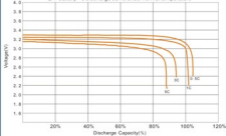
常溫下LYP鋰電池的放電特性曲線 LFP battery's discharge curve under normal temperature
