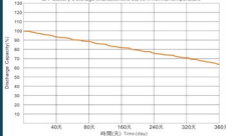
在常溫環境下LYP鋰電池的存儲特性曲線 LFP battery's storage characteristic curve in normal temperature
