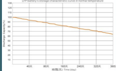
在常溫環境下LFP類電池的存儲特性曲線 LFP battery's storage characteristic curve in normal temperature
